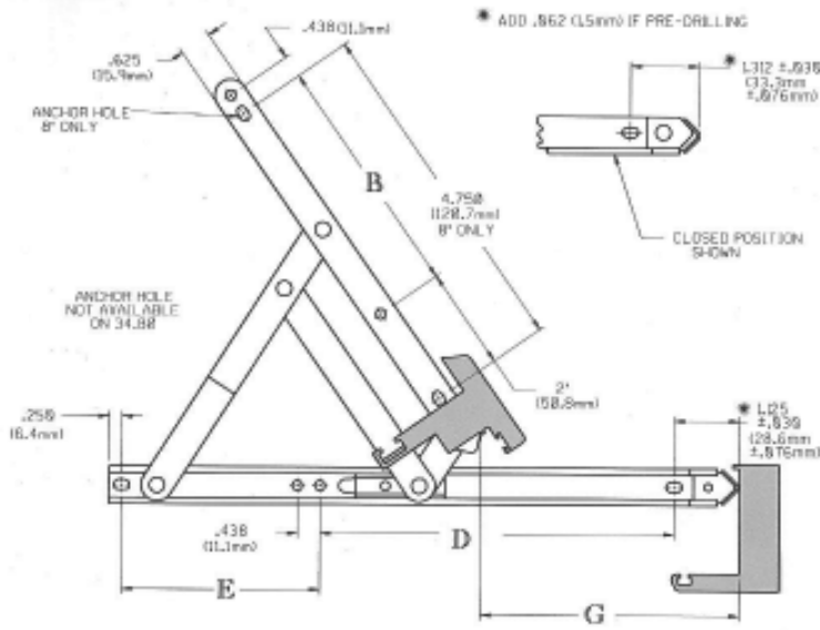
TRUTH STANDARD DUTY 4-BAR HINGE (Anderberg 201 Series)
