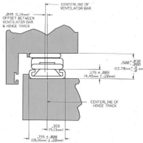
TRUTH STANDARD DUTY 4-BAR HINGE (Anderberg 201 Series)
